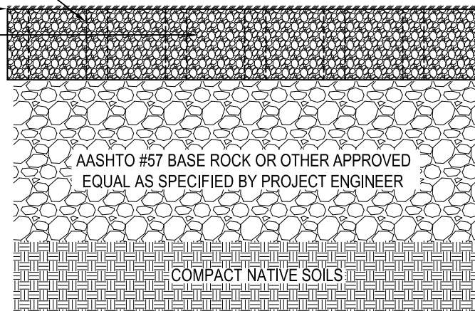
SECTION
