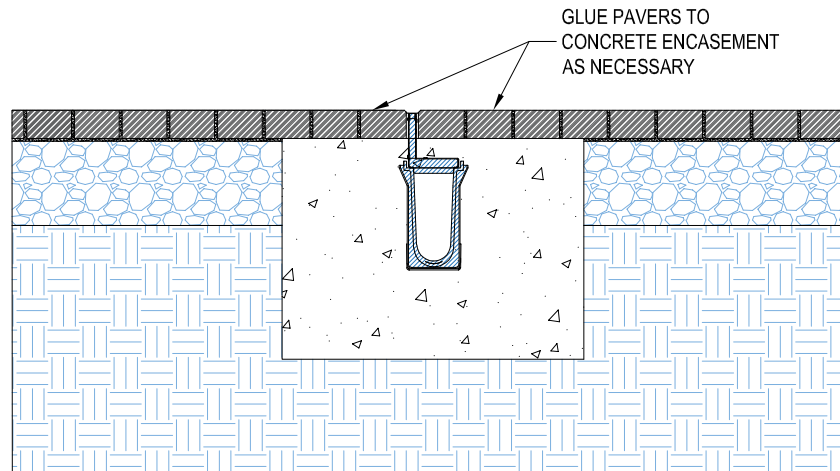
BRICK PAVER OR ASPHALT FINISH - CONCRETE ENCASEMENT HIDDEN
