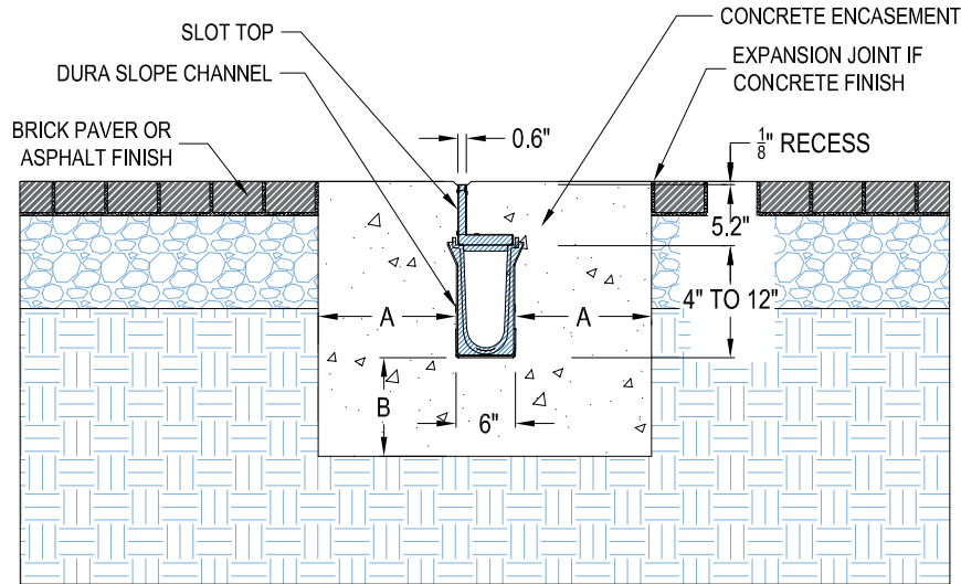
BRICK PAVER, ASPHALT FINISH, OR CONCRETE FINISH - CONCRETE ENCASEMENT VISIBLE
