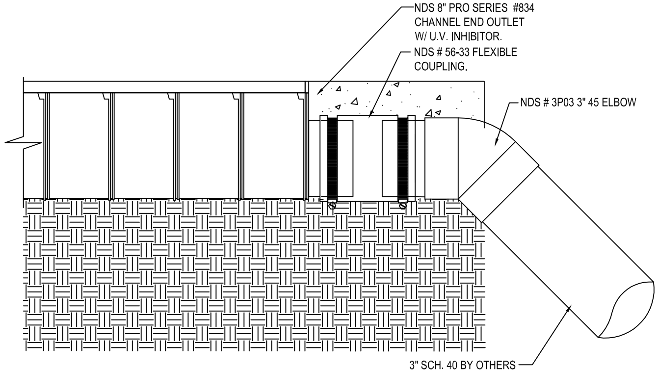
SECTION
