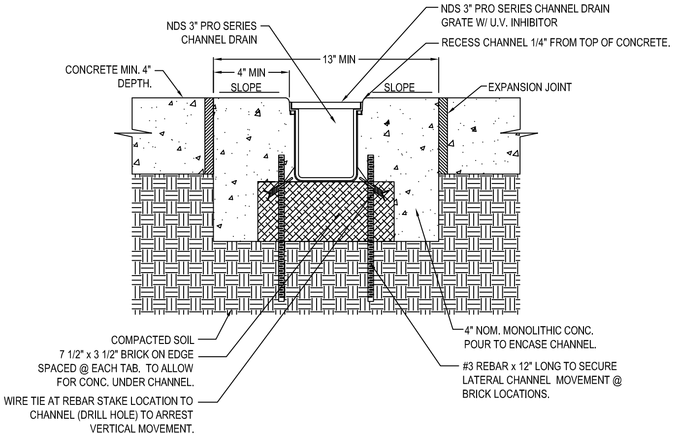
SECTION
